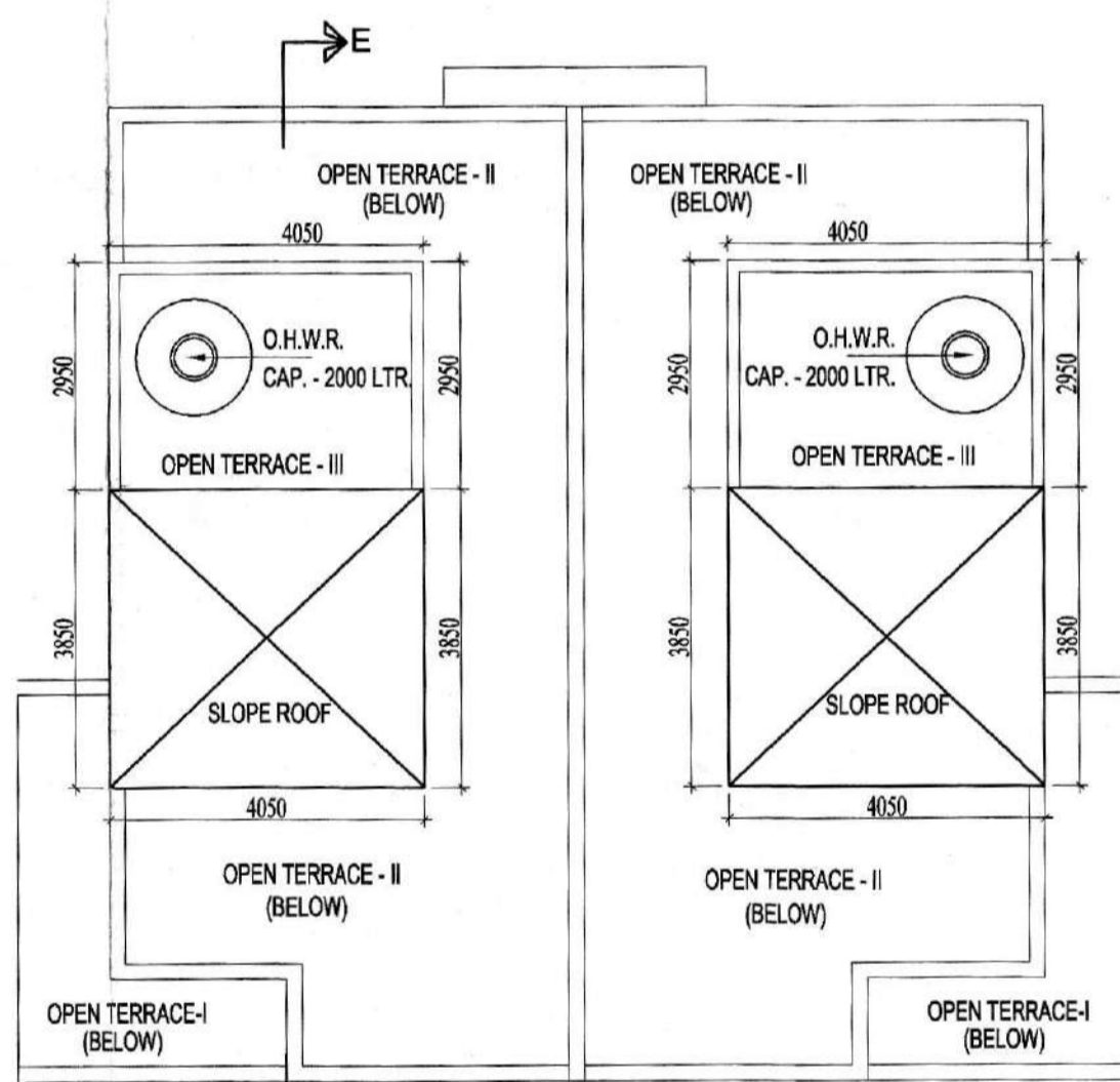
ROOF PLAN
